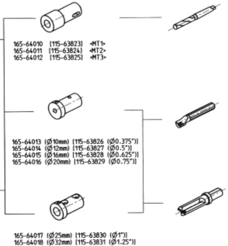
Combi toolholders for boring bars and insertdrill(s) Ø40 mm [Ø1.5"]
